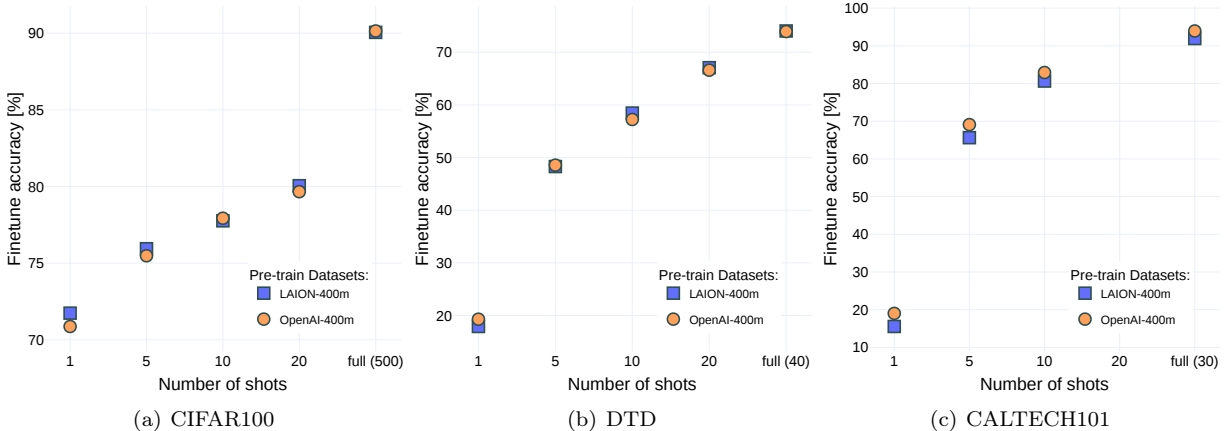
Figure 7: Effect of the pre-training data distribution: ViT instead of ResNet-50 While similar to Figure 14 the difference between the fine-tune performance is minimal, we observe that both models perform also very similarly in the few-shot setting. We hypothesize that this observation could be attributed to the similarity between LAION and OpenAI distributions rather than employing transformer instead of ResNet-50.
